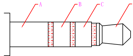
∅3.5 MATE PLUG
