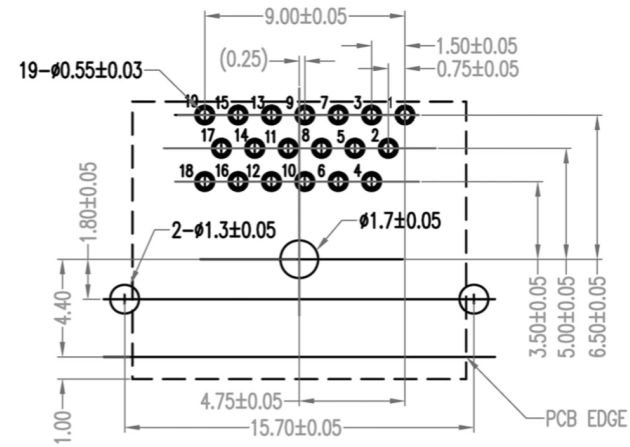
RECOMMENDED PCB LAYOUT SCALE 3:1
